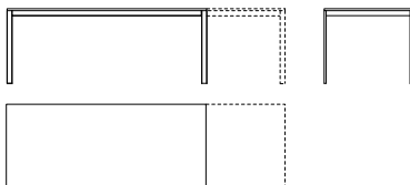
Fixed and extendable table L 123/203 P 79 H 75 cm W 48 3 / 8 /79" D 31 1 / 8 " H 29 4 / 8 "
